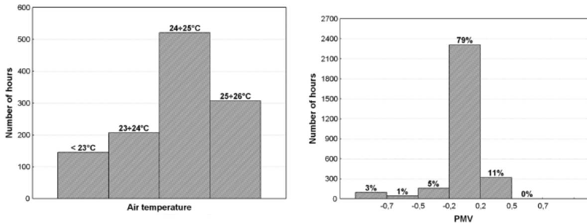
Figure 3. Histogram of the internal air temperature in the room (left graph) and the PMV index in the investigated room (right graph) – air supplied temperature: 20°C, the office faced south
