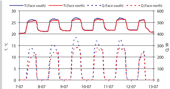
Figure 2. Time course of the temperature (Ti) in the office room provided with a cooling ceiling as the only source of cold and the additional demand for cooling power (Q) required to maintain a temperature of 24°C
