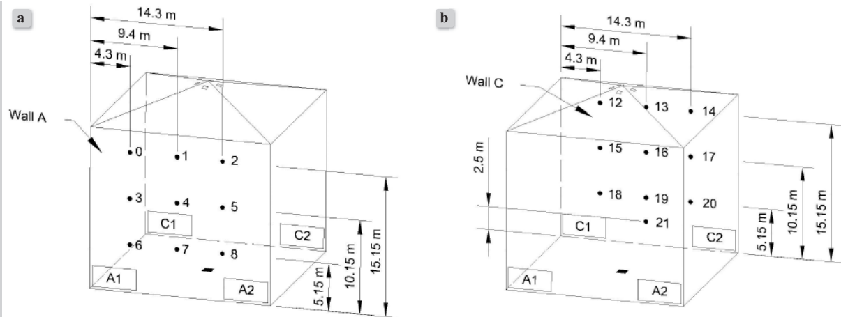
Figure 7. Layout of the sensors near the wall: a) wall A, b) wall C
